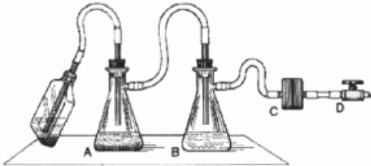
A. Collection Flask, B. Overflow Flask, C. Filter, D. Vacuum line
